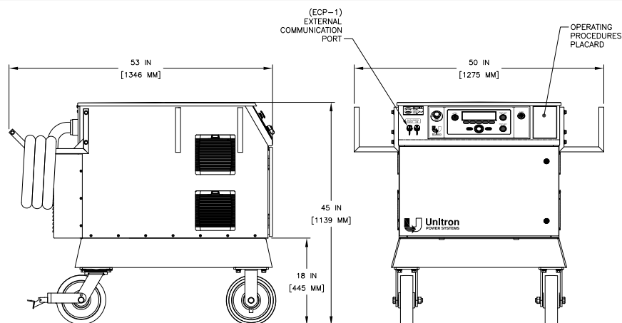
UFC SERIES PwrKart™ MOBILE GROUND POWER UNIT (GPU)
