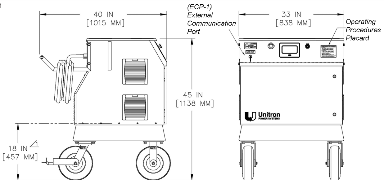
UFC SERIES PwrKart™ MOBILE GROUND POWER UNIT (GPU)
